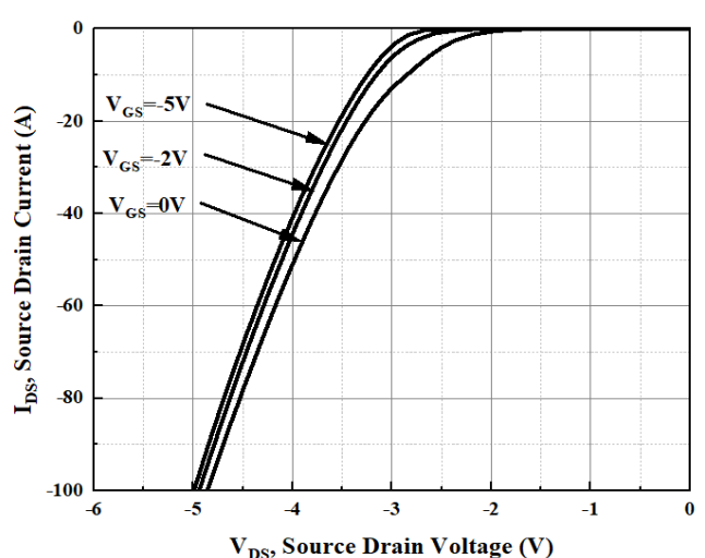
Figure 8. Body Diode Characteristic at Tj = 25 °C
